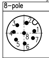
Contact arrangement
