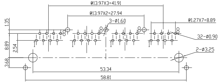
PC BOARD LAYOUT THICKNESS=1.6mm
