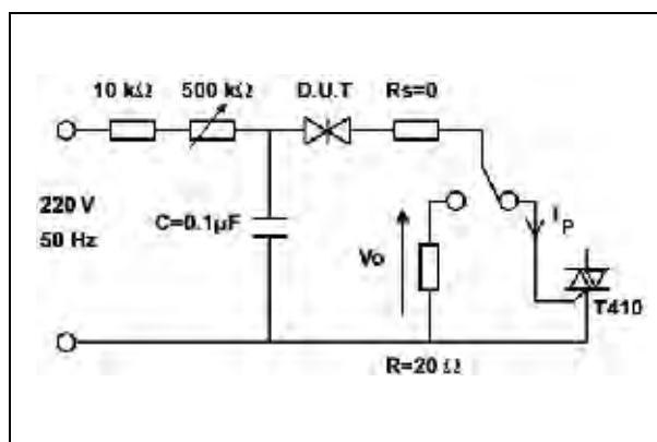
Diagram 2. Test circuit
