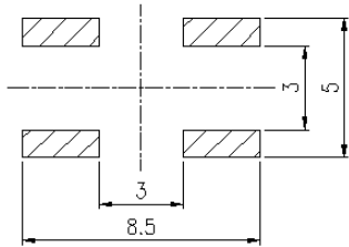
P. C. Board Dimension
