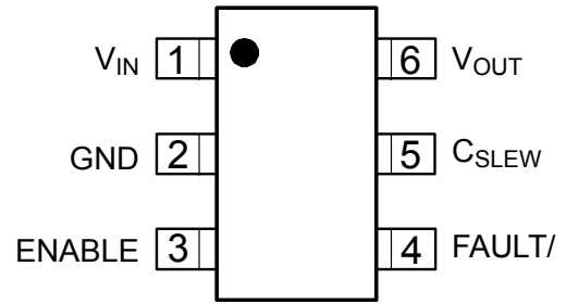
SOT 23-6 (M6) Top View
