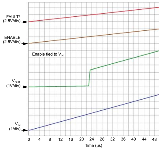
UVLO Increasing
