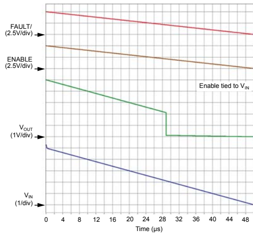
UVLO Decreasing
