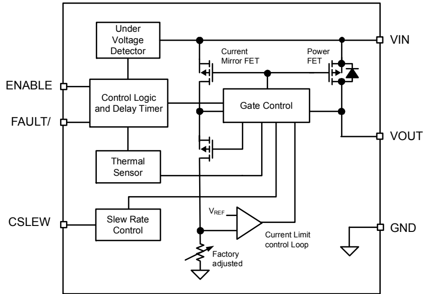
Figure 2. MIC2005/2015 Block Diagram
