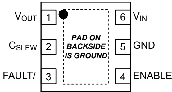
6-Lead 2mm x 2mm MLF (ML) Top View
