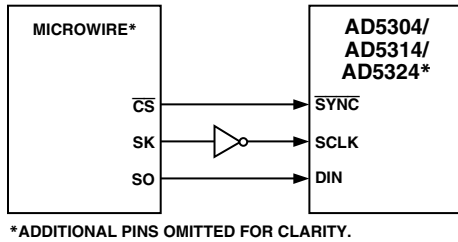
Figure 13. AD5304/AD5314/AD5324 to MICROWIRE Interface
