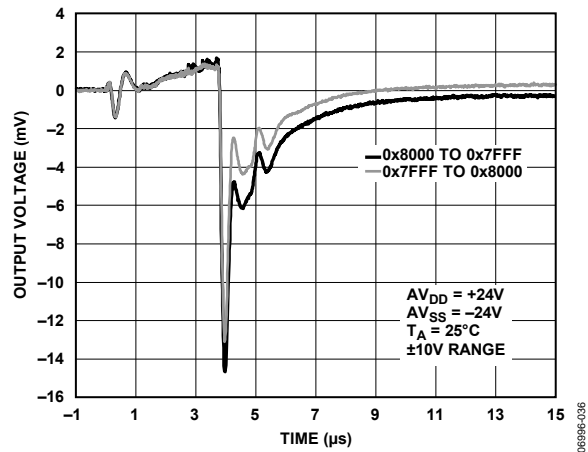
Figure 38. Digital-to-Analog Glitch
