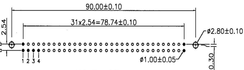
P.C. Board Layout
